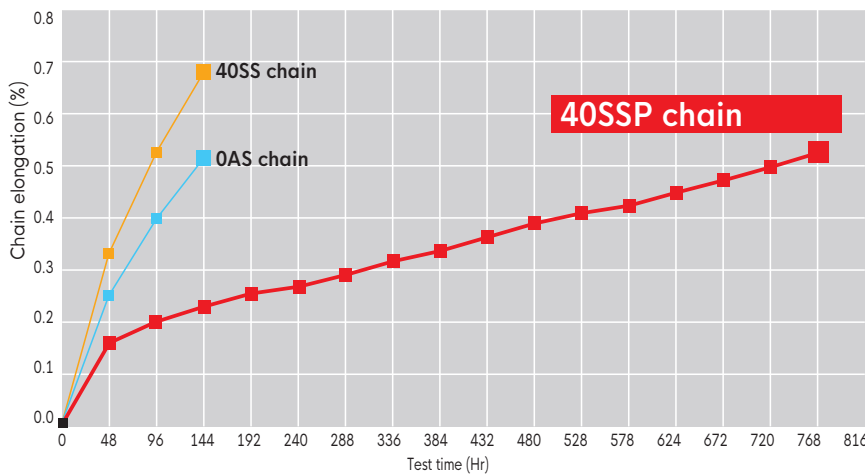
* SS, AS, and SSP were all tested under the same condition. Condition: load at 440N (maximum allowable tension for 40SS)
